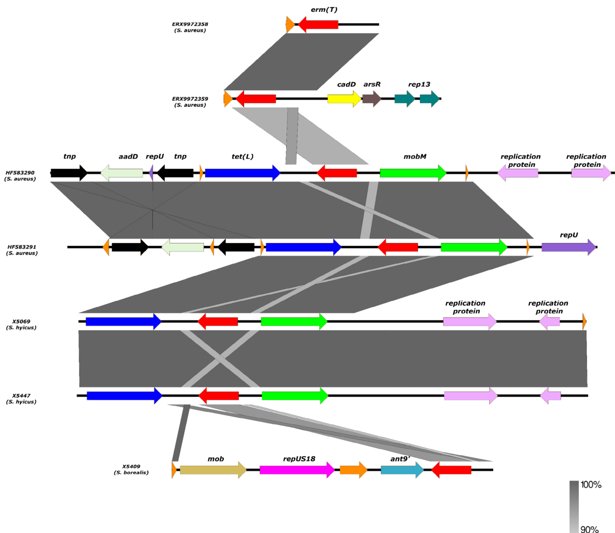
Fig. 3 Genetic environment of ermT gene of three CoNS isolates of this study (X5447, X5069, and X5409) in comparison with those of four reference strains
