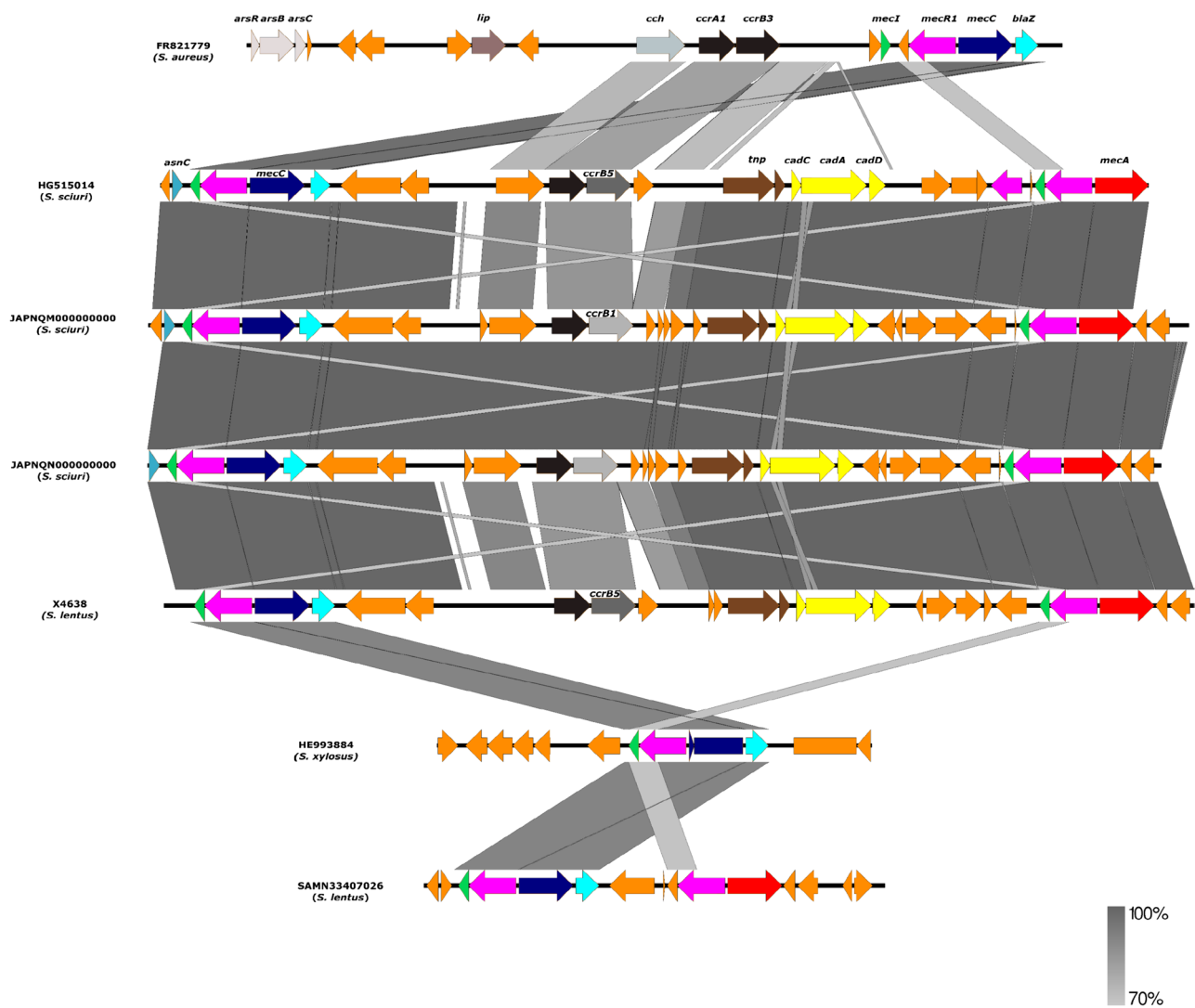
Fig. 4 The environment of the mecC gene of S. lentus (X4638) in comparison with previously described mecC -carrying coagulase-negative staphylococci and the S. aureus LGA251 strain
