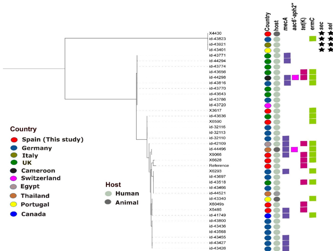
Fig. 1 Phylogenetic tree based on core genome SNP analysis of eight S. epidermidis isolates of this study with 31 publicly available genomes with similar lineages
