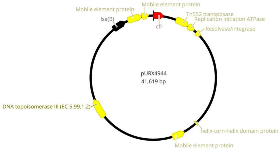
Fig. 5 Circular representation of the plasmid-carrying the cfr gene in S. saprophyticus
