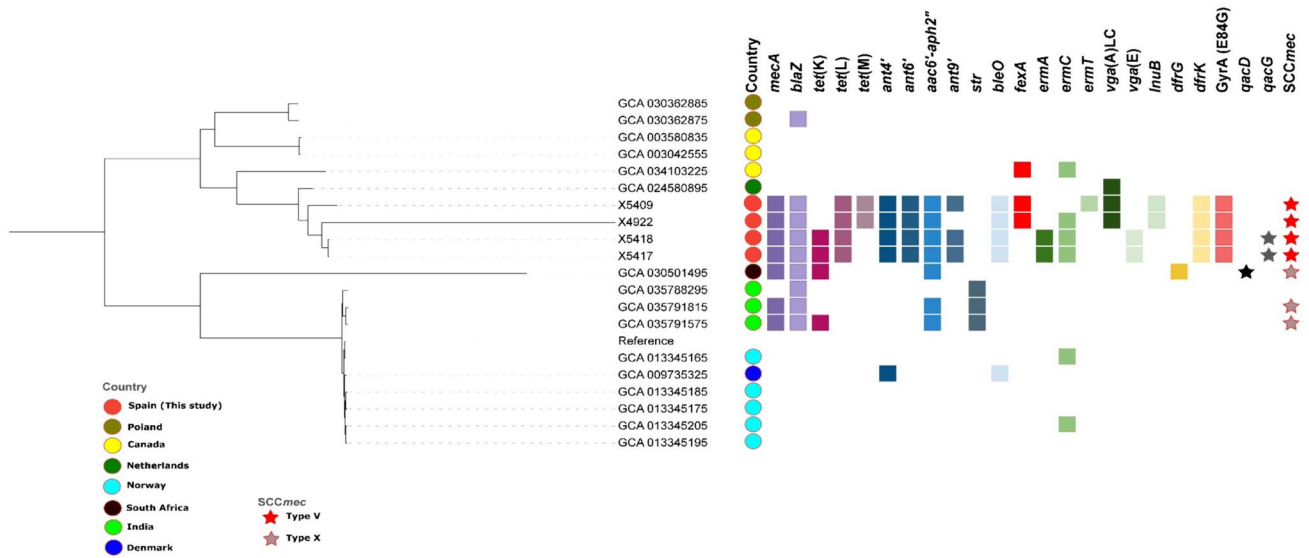
Fig. 2 SNIP-based phylogenetic tree of the four S. borealis isolates of this study mapped with all the 16 publicly available genomes
