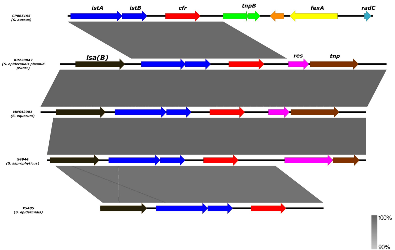
Fig. 6 Environment of the cfr gene of S. epidermidis (X5485) and S. saprophyticus (X4944) in comparison with previously described cfr -carrying coagulase-negative staphylococci and S. aureus
