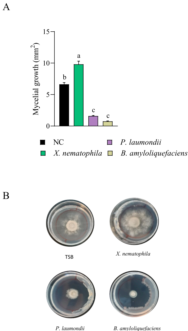
Fig. 3. Impact of Xenorhabdus nematophila , Photorhabdus laumondii , Bacillus amyloliquefaciens isolated bacteria in the Botrytis cinerea growth. (A) Mycelial growth (mm 2 ) of B. cinerea in the presence of X. nematophila , P. laumondii , and B. amyloliquefaciens isolated bacteria. (B) Display of the fungal growth in each treatments four days after infection. Data are expressed as mean \pm SEM. Different lowercase letters represent statistically significant differences between treatments according to Tukey's multiple comparison test ( P < 0.05 ).
