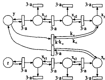
Figure 13. PN modelling a third order delay.
