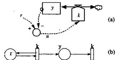
Figure 8. a) DF modelling a simple storage system, b) its equivalent PN.
