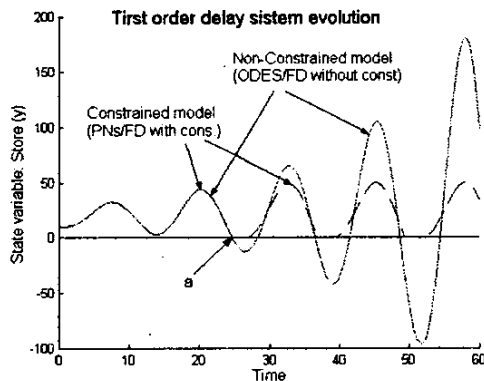
Figure 14. First order delay system evolution in constrained and non-constrained models.
