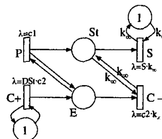
Figure 6. ISSCPN equivalent to the system in Figure 4 restricted to positive values.
