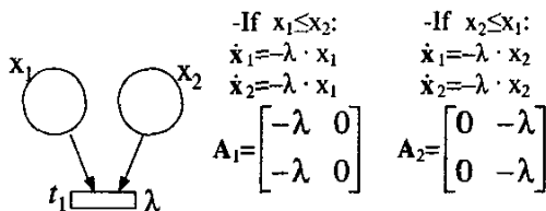
Figure 2: A ISSCPN whose associated linear systems have non Metzler matrices.
