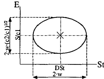
Figure 5. Behaviour of the system described in Figure 4
