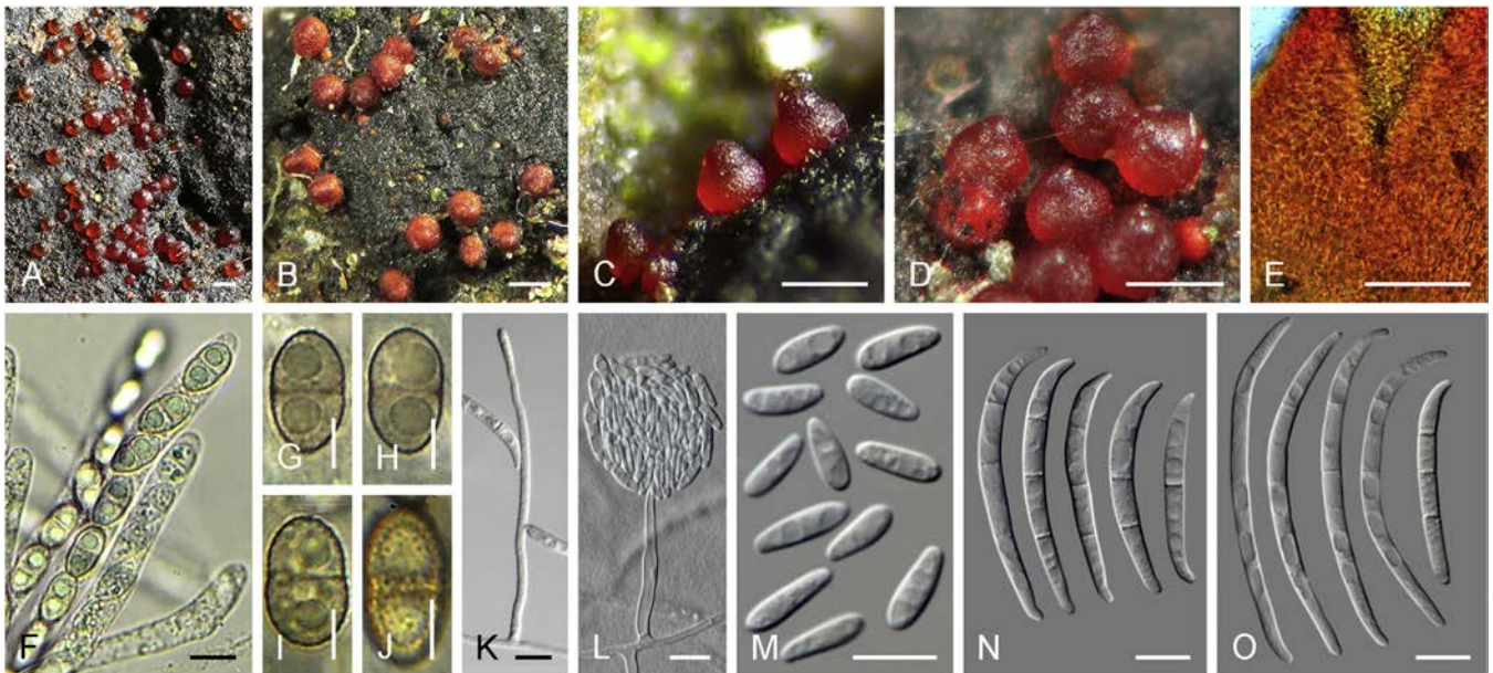
Fig. 19. Cosmospora spp. A–D. Ascomata on natural substrate. E. Surface view of perithecial wall. F. Asci. G–J. Ascospores. K, L. Conidiophores. M, N, O. Macroconidia. A–J. “ Cosmospora ” flavoviridis (photos P. Mlčoch). K–N. “ Cosmospora ” flavoviridis (CBS 124353). O. Cosmosporella cavisperma (CBS 172.31). Scale bars: A–D = 300 \mu m; E = 50 \mu m; G–J = 5 \mu m; all others = 10 \mu m.
