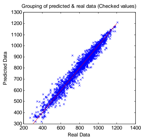
Figure 7: grouping of predicted data, opposed to real checked values.
