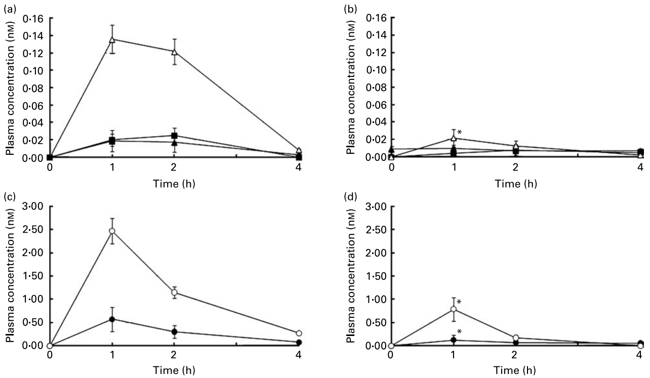
Fig. 2. Pharmacokinetic curves of monomeric forms, (—■—) catechin, (—△—) epicatechin (—▲—) and epicatechin gallate (a and b), and polymeric forms, (—●—) dimer and (—○—) trimer (c and d), detected in rat plasma collected between 0 and 4 h after the ingestion of grape seed procyanidin extract with and without carbohydrate-rich food. The results are expressed as nm. * Mean value was significantly different from that without carbohydrate-rich food ( P < 0.05 ; unpaired Student's t test).
