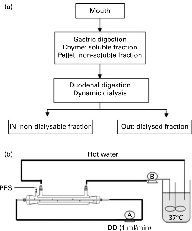
Fig. 1. (a) Steps of the proposed in vitro digestion model. (b) Schema of the duodenal digestion with dynamic dialysis. DD, duodenal mixture (fraction found inside dialysis solution (IN)); PBS (fraction found outside dialysis solution (OUT)).
