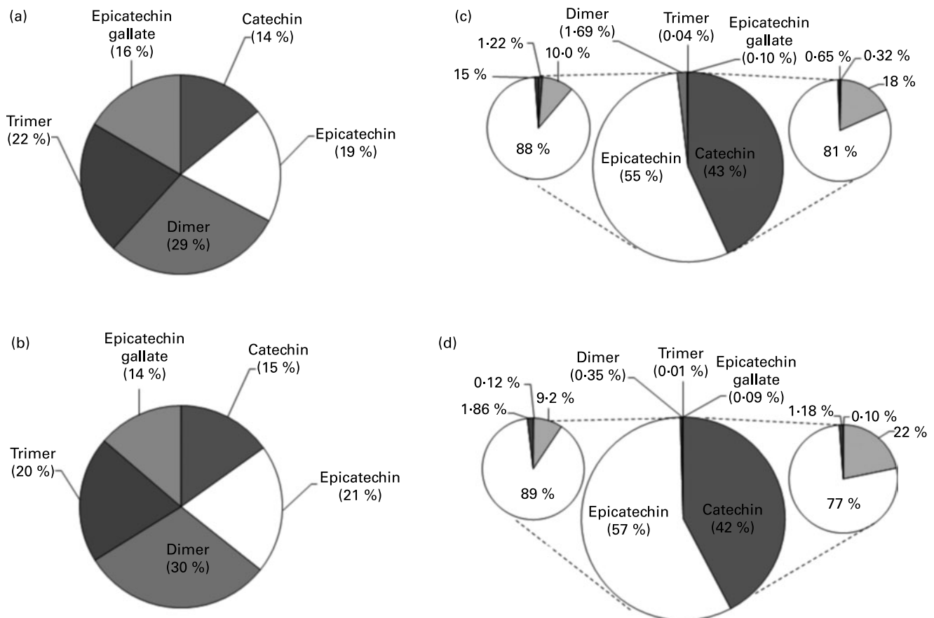
Fig. 4. (a and b) In vitro and in vivo grape seed procyanidin extract (GSPE). Percentage of the catechin, epicatechin, epicatechin gallate, dimer and trimer in the dialysed fraction (fraction found inside dialysis solution) of the duodenal mixture. (c and d) In vitro and in vivo GSPE + carbohydrate-rich food. Percentage of the catechin, epicatechin and their respective metabolites, epicatechin gallate, dimer and trimer in the postprandial rat plasma.
