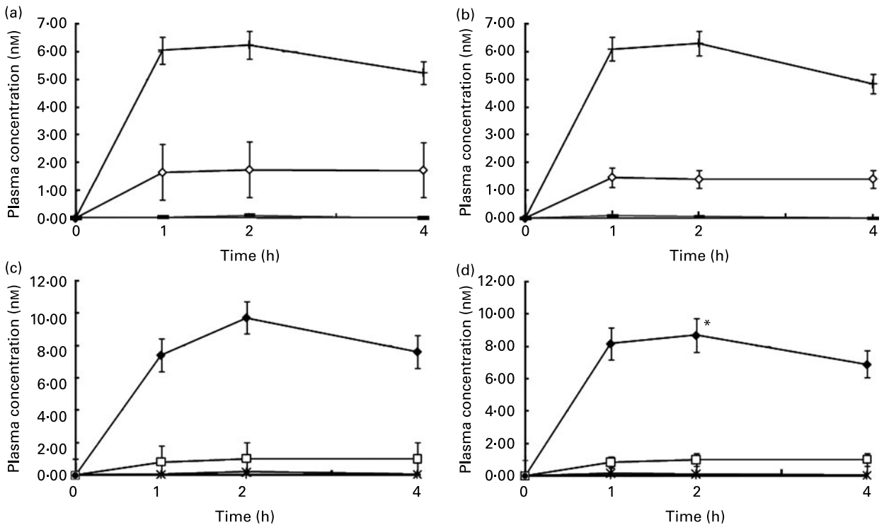
Fig. 3. Pharmacokinetic curves of grape seed procyanidin extract (GSPE) metabolites according to the monomer structure, being (—◇—) catechin methyl glucuronide, (—+—) catechin glucuronide and (—■—) catechin methyl sulphate (a and b), and (—□—) epicatechin methyl glucuronide, (—◆—) epicatechin glucuronide and (—*—) epicatechin methyl sulphate (c and d), detected in rat plasma collected between 0 and 4 h after the ingestion of GSPE with and without carbohydrate-rich food. The results are expressed as nm. * Mean value was significantly different from that without carbohydrate-rich food ( P < 0.05 ; unpaired Student's t test).
