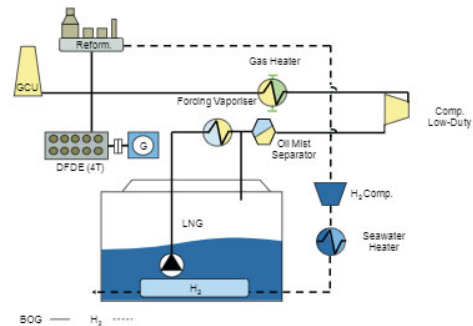
Fig. 7. Pressurised H 2 storage
