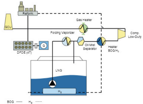
Fig. 9. Cooled H_2 storage
