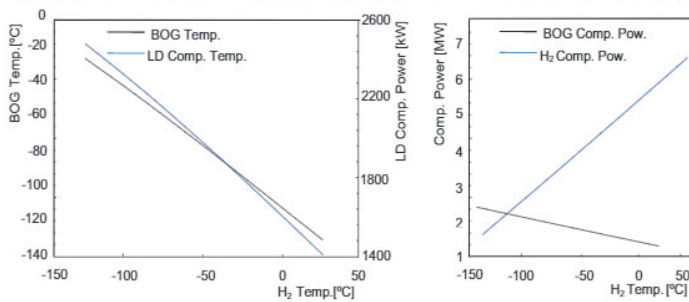
Fig. 13. Effect of H_2 temperature variation: (a) Comparison between BOG temperature, H_2 temperature and LD power; (b) Comparison between H_2 temperature and compressor power
