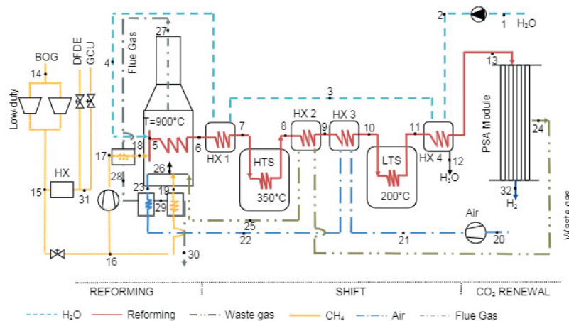
Fig. 3. Reforming process using steam from the excess BOG generated in the tanks of an LNG vessel
