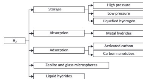
Fig. 6. H 2 storage methods
