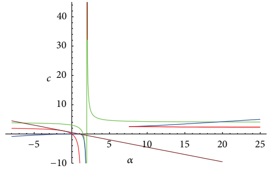
FIGURE 4: Bifurcation curves of critical points.
