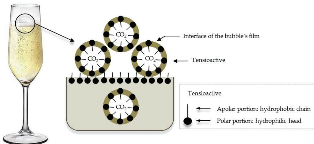
Figure 1. Carbon dioxide/liquid interphase of the bubble's film. Adapted from Ref. [11].
