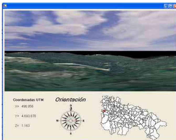
Fig. 12. User interface
