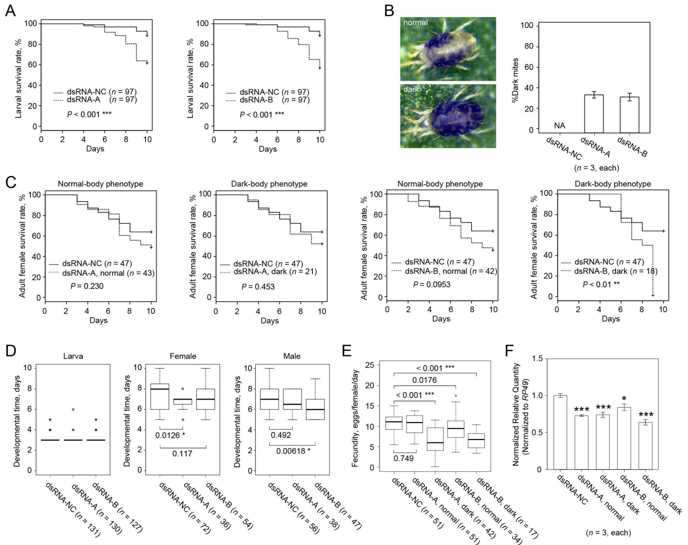
Fig 5. The effect of dsRNA- TuVATPase delivered by the leaf coating method. (A) Larval survivorship when feeding on bean leaf discs coated with the solution of dsRNA- TuVATPase -A, dsRNA- TuVATPase -B (dashed lines) or dsRNA-NC (solid line). Data were collected from 3 independent experimental runs. Survival curves were plotted using the Kaplan–Meier method and compared using the log-rank test with Bonferroni correction (***, P < 0.001/2 ). (B) Normal and dark-body female mites, and frequency of phenotypes observed after feeding on leaf discs coated with the solution of dsRNA- TuVATPase -A, dsRNA- TuVATPase -B or dsRNA-NC. The bar graph represents dark-body mite frequencies collected from 3 independent experimental runs. (C) Survivorship of adult female mites upon feeding on bean leaf discs coated with the solution of dsRNA- TuVATPase -A, dsRNA- TuVATPase -B (dashed lines) or dsRNA-NC (solid line) for normal and dark-body mites respectively. Data were collected from 3 independent experimental runs. Survival curves were plotted using the Kaplan–Meier method and compared using the log-rank test with Bonferroni correction (no asterisk, P > 0.05/4 ; **, P < 0.01/4 ). (D) Developmental times of the larval and adult female and male mites. Data were collected from 3 independent experimental runs and were compared using the Wilcoxon–Mann–Whitney test with Bonferroni correction (no asterisk, P > 0.05/2 ; *, P < 0.05/2 ; **, P < 0.01/2 ). (E) Normal and dark-body mite fecundity. Data were collected from 3 independent experimental runs and were compared using the Wilcoxon–Mann–Whitney test with Bonferroni correction (no asterisk, P > 0.05/4 ; ***, P < 0.01/4 ). (F) TuVATPase gene expression relative to the expression of RP49 reference gene in normal and dark-body female mites. Data were represented as mean \pm SE and analysed using the Dunnett’s test (*, corrected P < 0.05 ; ***, corrected P < 0.001 ).
