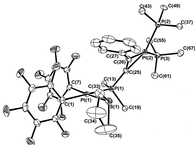
Figure 2. View of the molecular structure of [(C 6 F 5 ) 2 (tht)Pt( \mu -1 \kappa P:2 \eta^2 -PPh 2 C≡CPh)]Pt(PPh 3 ) 2 , 3a . Ellipsoids are drawn at the 50% probability level. Hydrogen atoms have been omitted for clarity, and the phenyl groups bound to the phosphorus atoms are represented by their ipso -carbons only.
