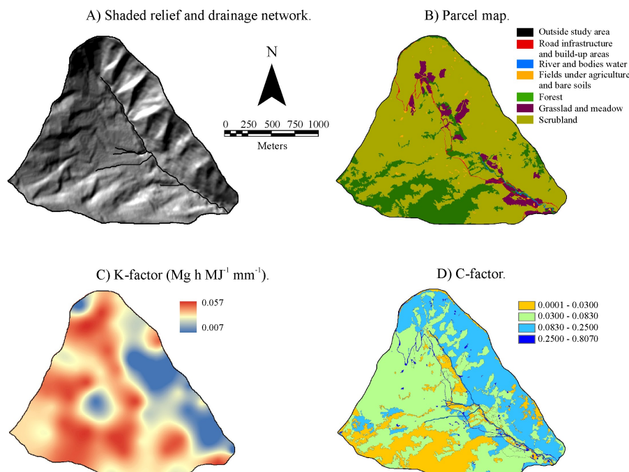
Fig. 2. Input data derived from the database of the Arnás catchment: (A) drainage network map derived from the DTM using threshold value of 1 \text{ km}^2 contributing area (continuous line); (B) parcel map, derived from the current land use/land cover map; (C) soil erodibility map (K-factor in RUSLE, \text{Mg h MJ}^{-1} \text{ mm}^{-1} ); and (D) crop management map (C-factor in RUSLE).
