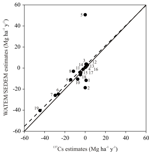
Fig. 4. Results of the calibration process: comparison of WATEM/SEDEM and 137 Cs soil redistribution estimates for the best parameter set. The solid lines represents a perfect fit, and the dashed one is the linear regression between both datasets.
