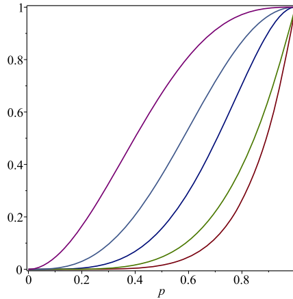
Fig. 5. Plots of P_k(p) , k = 1, \dots, 5 , from left to right, respectively.
