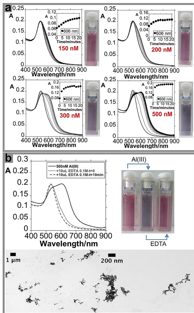
Figure 3. Spectrophotometric titration of AuNPs@TC with the addition of increasing amounts of Al(NO 3 ) 3 and naked-eye detection (a). Reversible colorimetric change upon addition of EDTA in aqueous solution and TEM images of AuNPs@TC with the addition of 500 nM of Al(NO 3 ) 3 (b).
