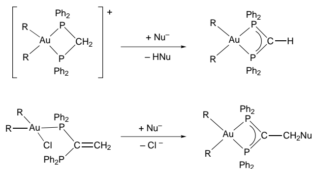
Scheme 1 R = \text{C}_6\text{F}_5
